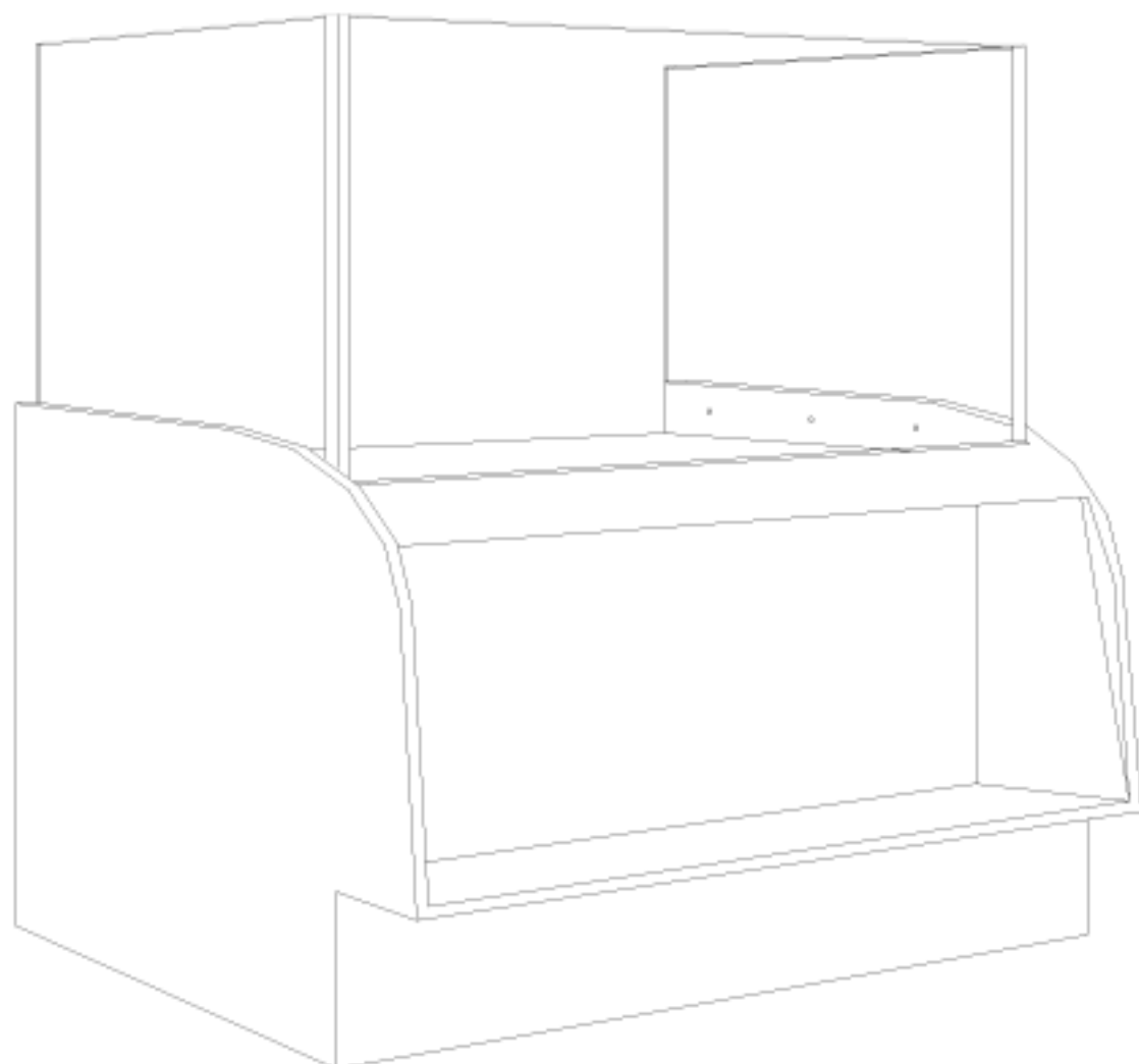
93440-59 Front
